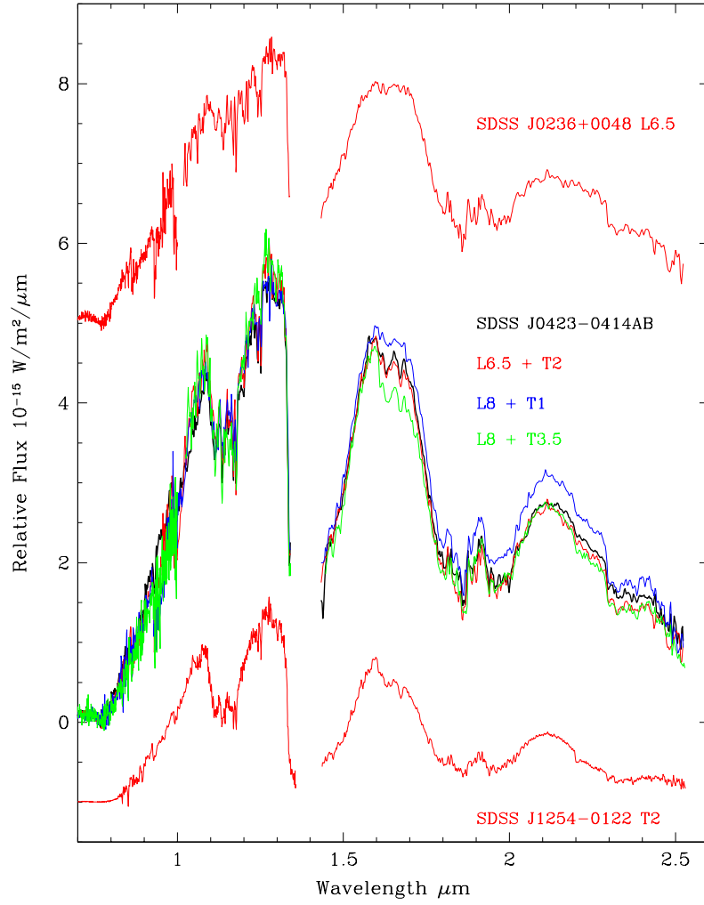
FIG. 2.— Comparison of red optical and near infrared spectral data for SDSS 0423-0414 (center, in black) to various pairings of late-type L and T dwarf spectra. The best match of a combined L6.5 (top) and T2 (bottom) is shown overlain on the spectrum of SDSS 0423-0414 in red. In contrast, later-type primaries (e.g., L8+T1 in blue) and secondaries (L8+T3.5 in green) yield poor agreement in band strengths and/or H - K color. Earlier-type primaries and later-type secondaries fail to reproduce the absolute magnitudes of the components.
